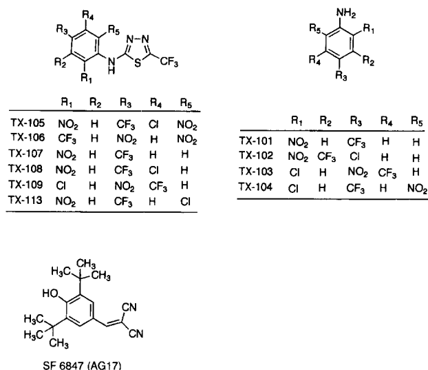
Figure 1. Chemical structures of thiadiazolylanilines and SF 6847 (AG17).
